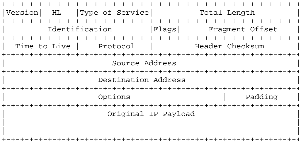
Figure 1: GRE Encapsulation Frame Format
