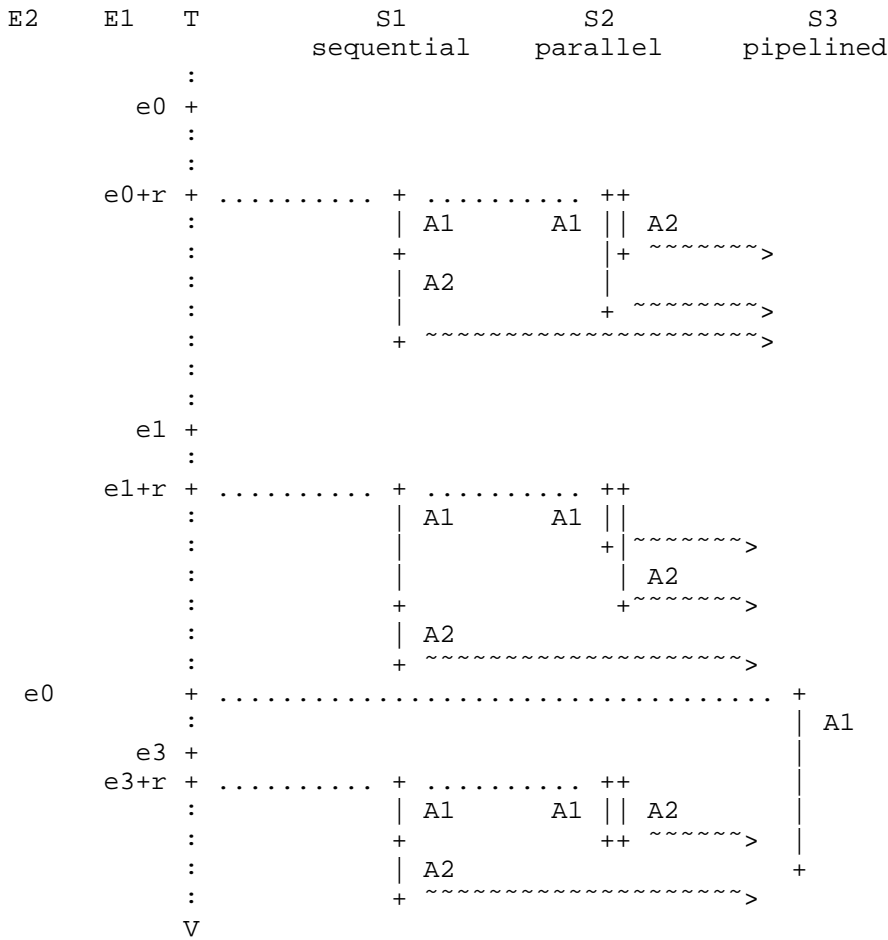
Figure 2: Example Execution
