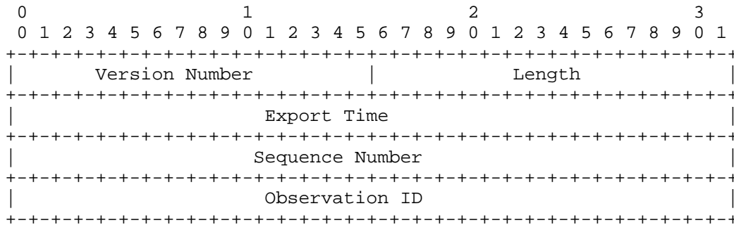
Figure 5: IPFIX Message Header
