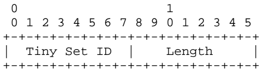
Figure 11: TinyIPFIX Set Header
