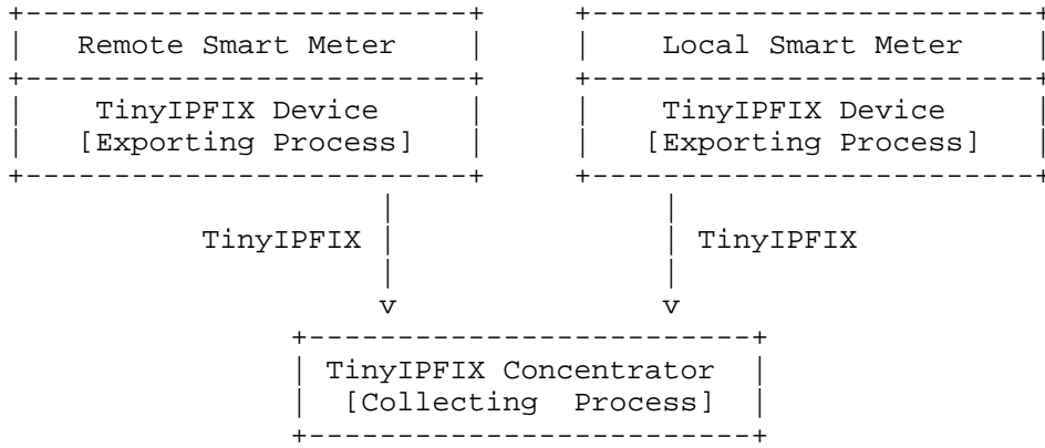
Figure 3: TinyIPFIX Mediator
